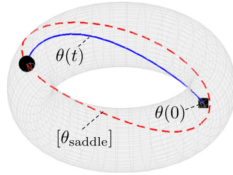
(b) Trajectory \theta(t) for \kappa = 1 .
