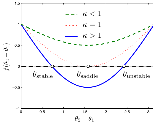
(a) Vector field in Eq. (15).
